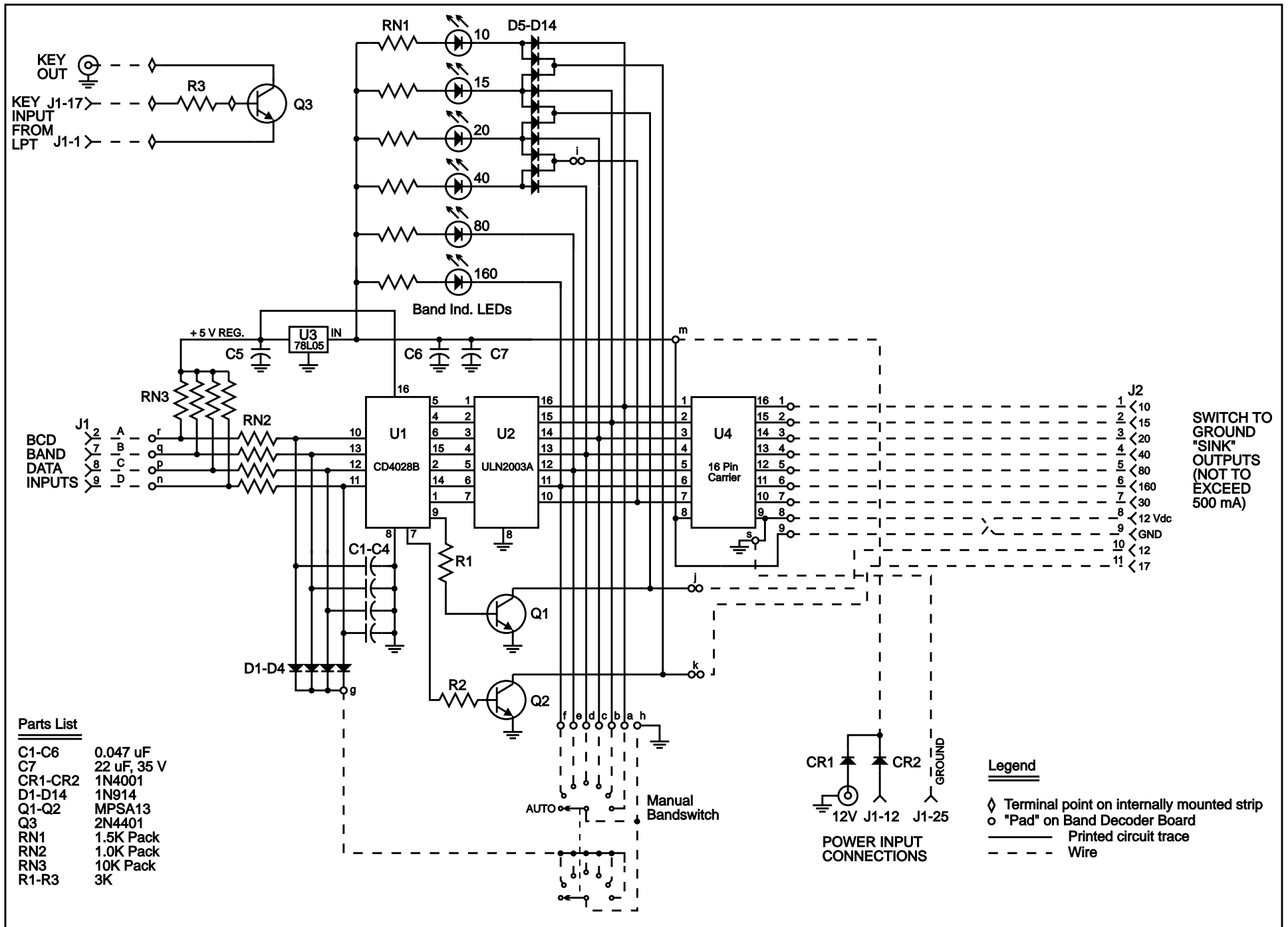
Figure 1a - Band Decoder Schematic for Yaesu Radios or Computer LPT Control - Basic Model (No Source Driver Modification)
