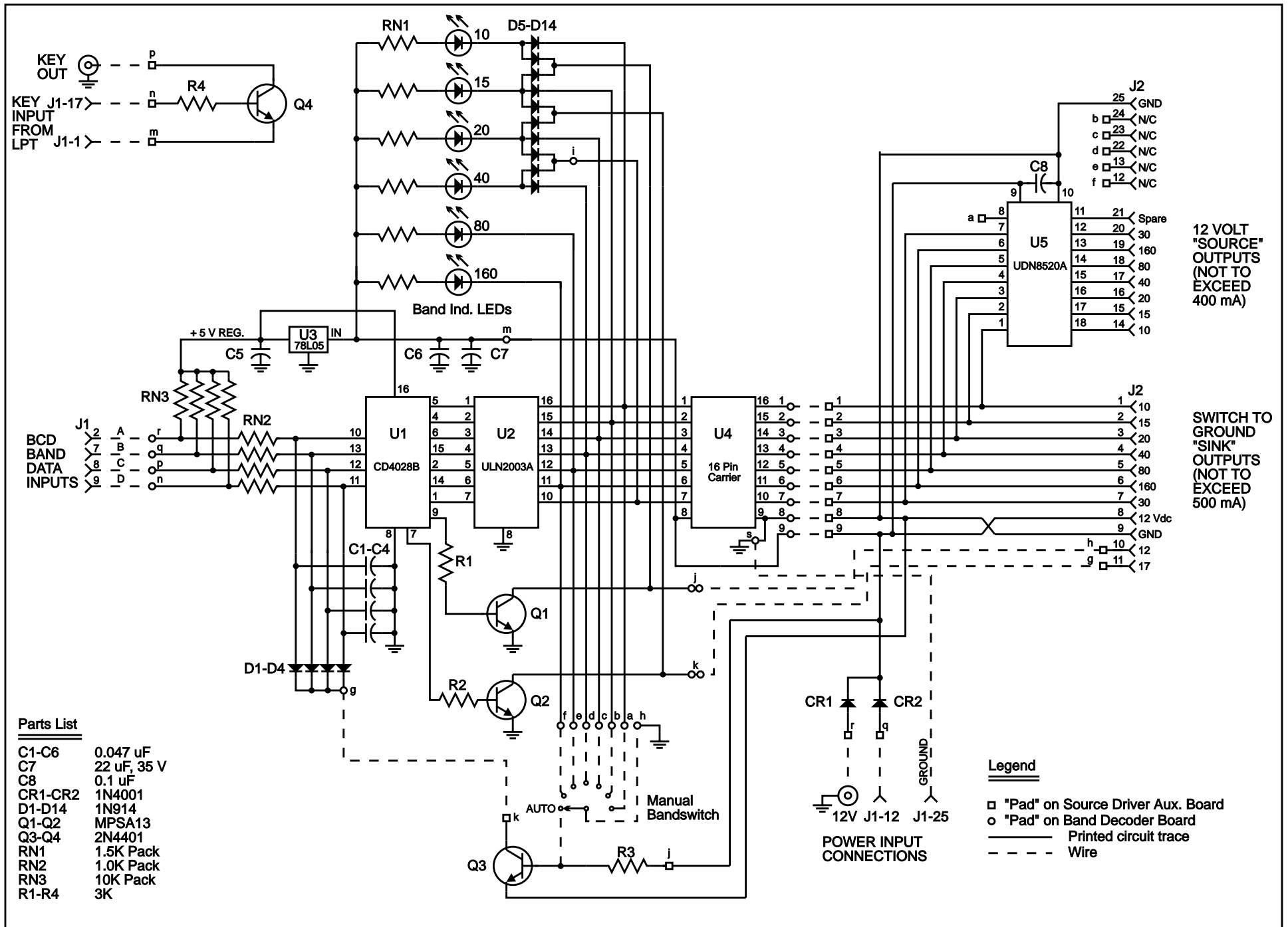
Figure 1 - Band Decoder Schematic for Yaesu Radios or Computer LPT Control
