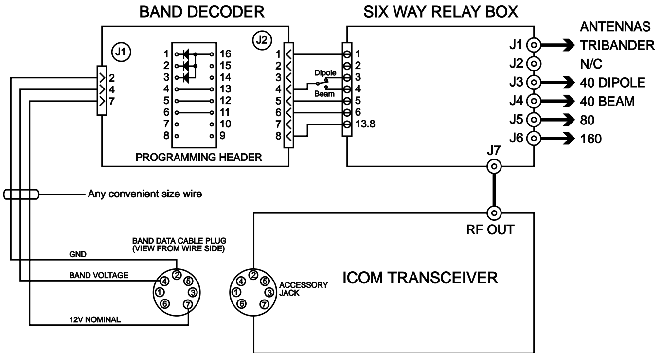
Figure 2c - Tribander, Two 40 Meter Antennas, Plus Monoband Antennas on 80 and 160 . The transceiver provides power for decoder and relays as well as the band data information. Three diodes installed on the programming header select Six Way Relay No. 1 (Output J1) whenever the rig is on 10, 15, or 20. An external toggle switch selects between the two available 40 meter antennas. Three internal jumpers are installed to select the monoband antennas for 40-160 meters.
