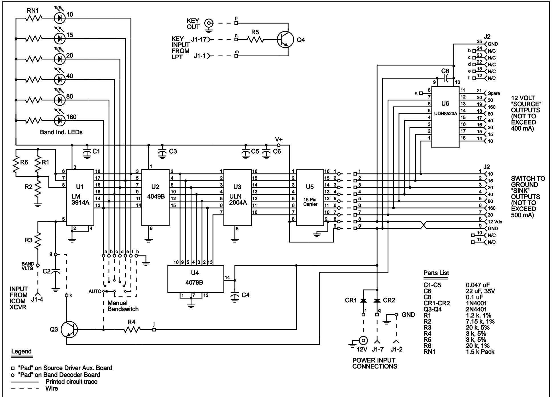
Figure 1 - Band Decoder Schematic for Icom Radios
