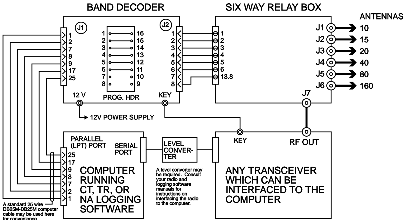
Figure 3a - Monoband Antennas . Similar to Figure 2a, except that the band data comes from the computer. 12 Vdc power for the decoder and relays comes from an external supply. Consult your logging software for instructions on enabling band data on LPT ports. NA sends band data to different LPT port pins than does CT and TRLog. Consult your manual. Transmitter CW keying is provided by a transistor in the decoder if CT is running on the computer.
